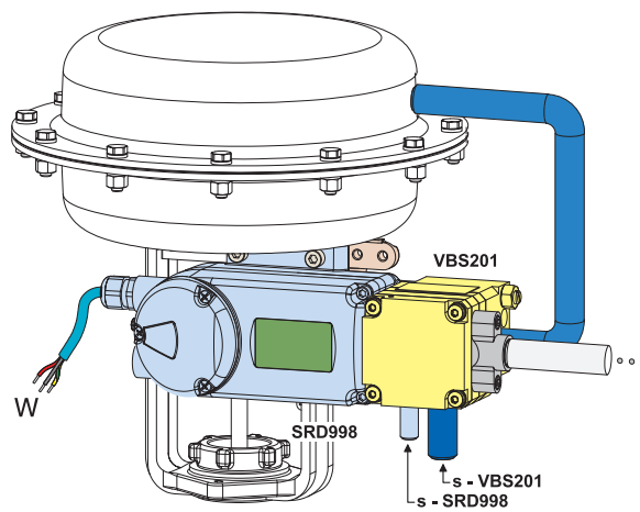
Figure 4. Mounting Example 1
