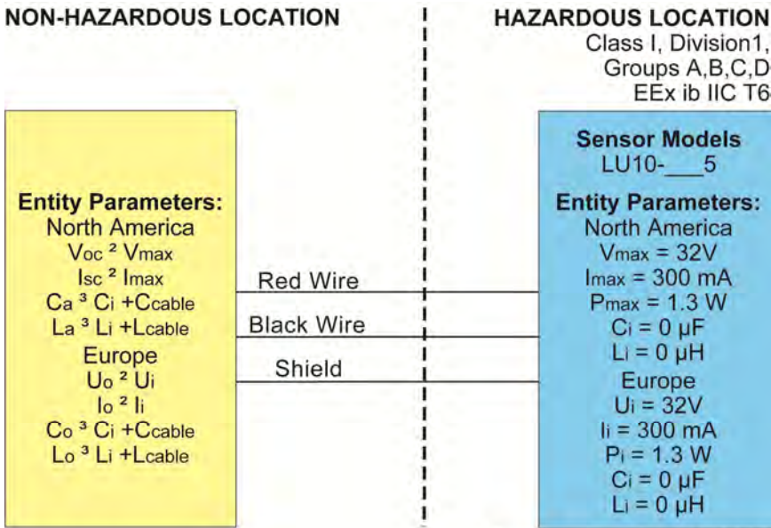
Sensor Drawing: U10900 Sheet 1 of 2 Rev. B 4-02-01
