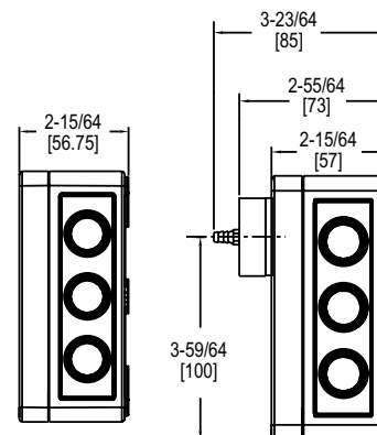
Duct mount
