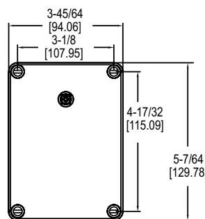
Wall mount
