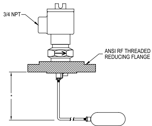
Vertical, flange installation
