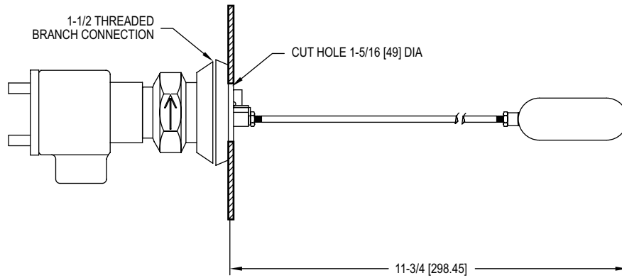
Standard installation
