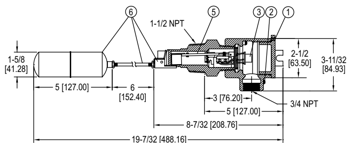
ATEX/IECEX unit
