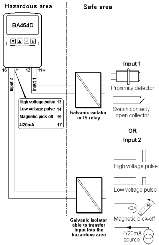
Fig 7 Batch controller protected by galvanic isolators with input in the safe area.
