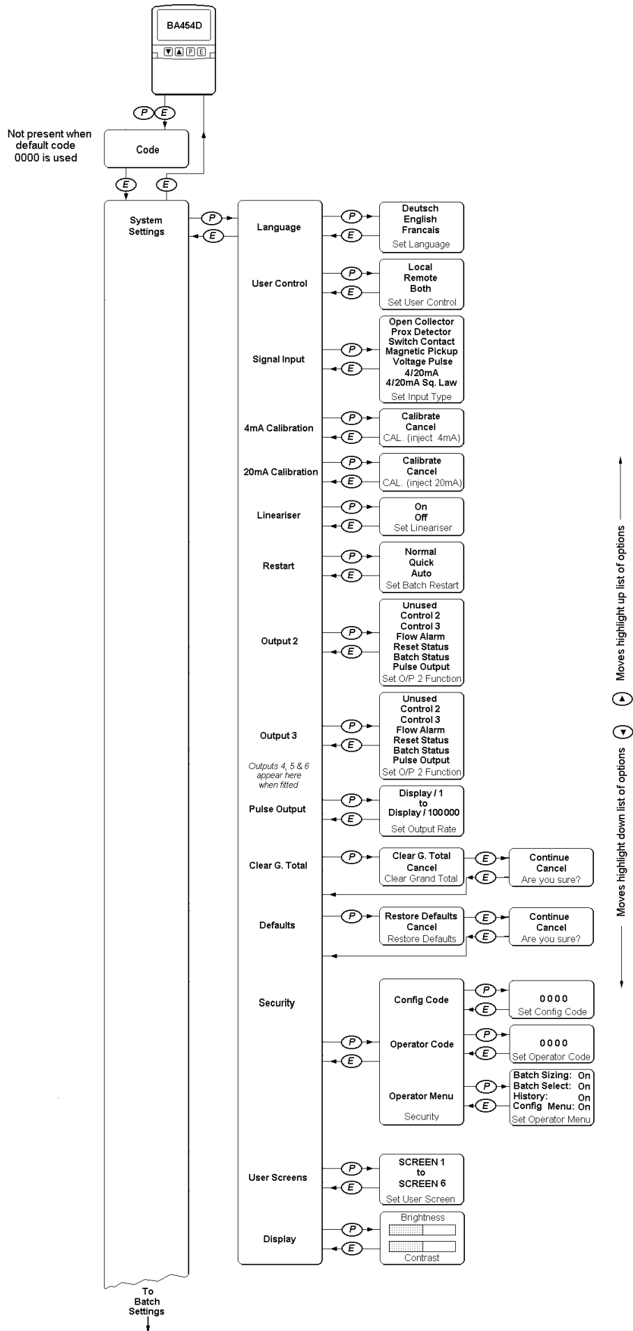
Fig 11 System Settings
